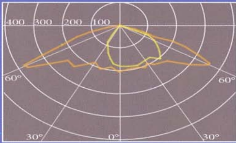
Polar Diagram
